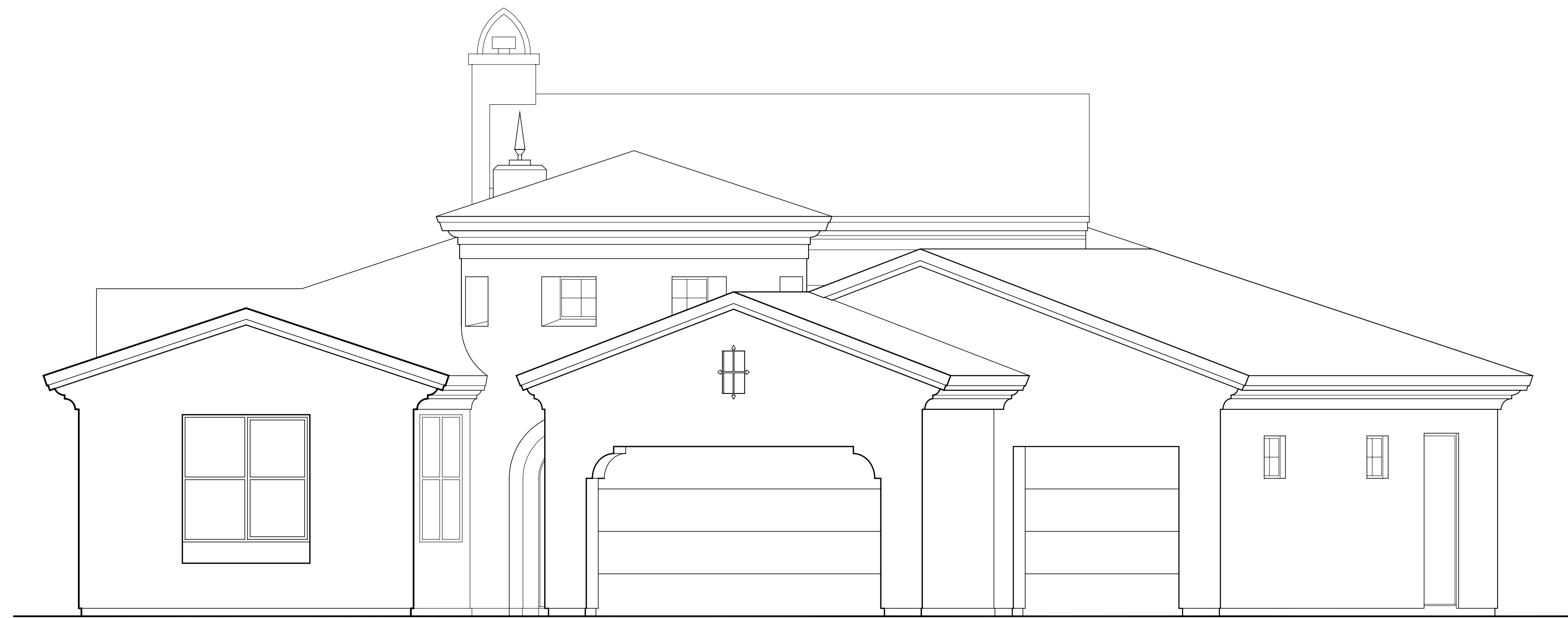
1 FRONT ELEVATION
